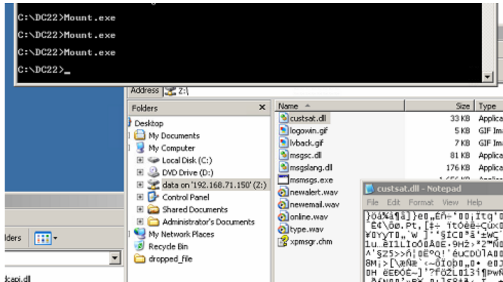
Figure 4. Snapshot of HDDCryptor's encryption routine to mapped drives
